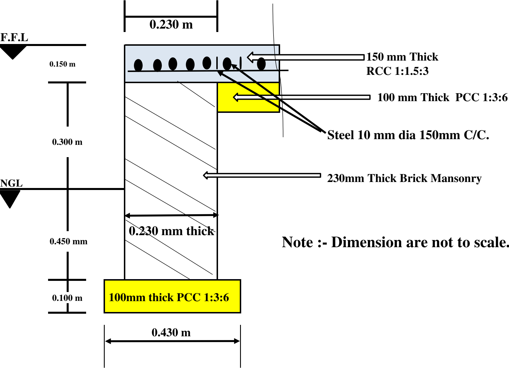
Section C-C
