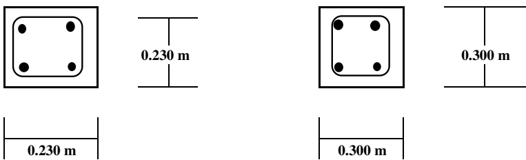
Plan P2
