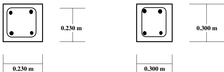
Plan P2
