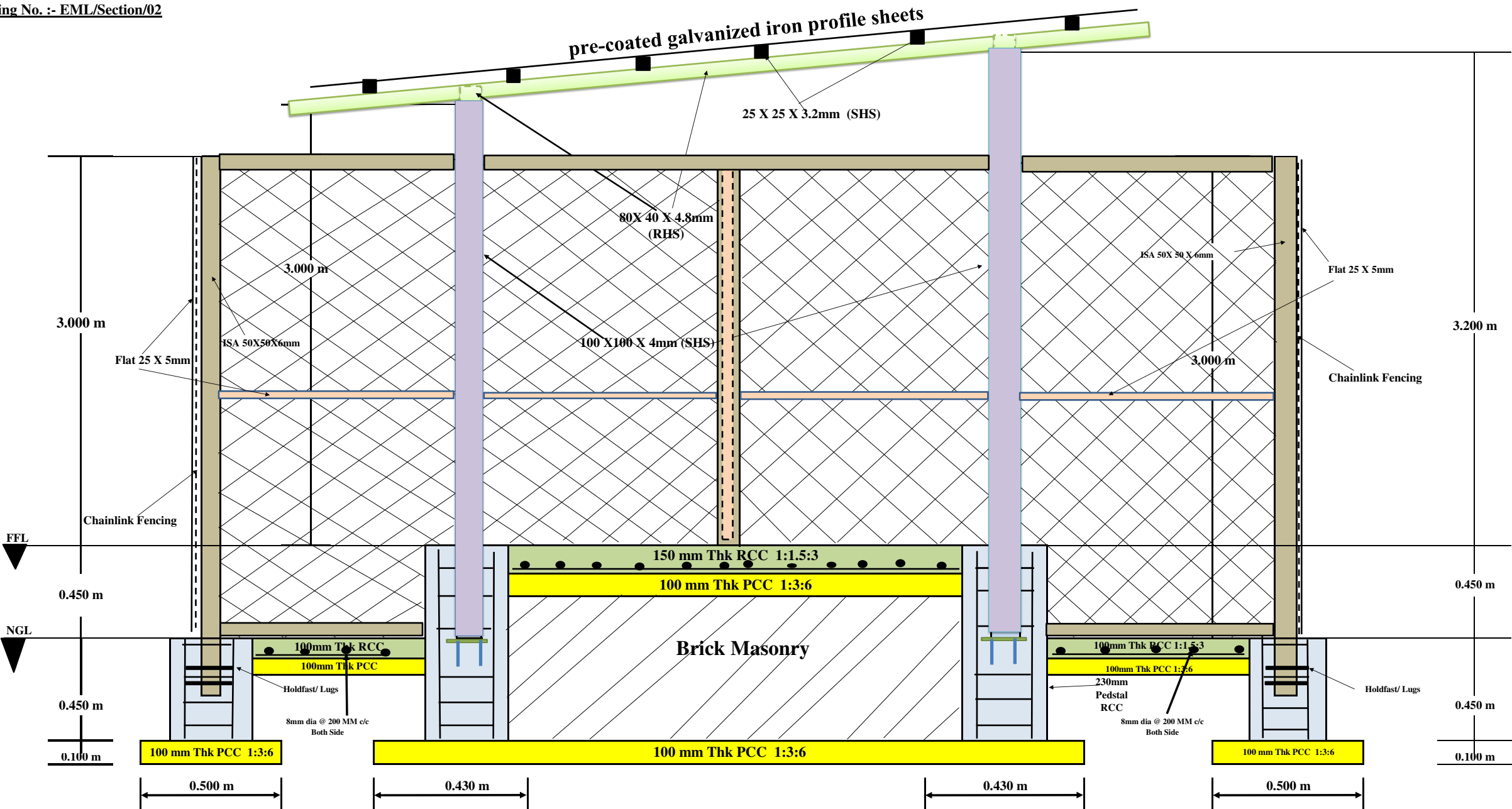
Section B-B
