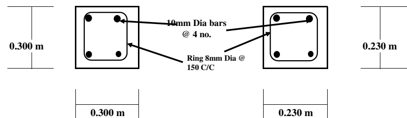
Plan P1
